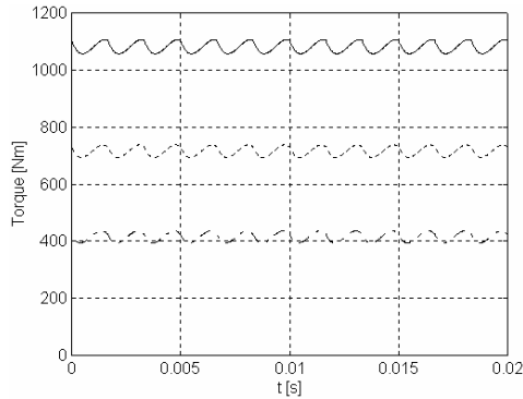
f) Itnea, U_1 = U_{1N} ; f_1 = 50\text{Hz}
