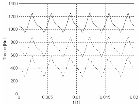
d) Itnnf1, U_1 = U_{1N} ; f_1 = 50\text{Hz}
