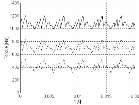
a) Impea, U_1 = U_{1N} ; f_1 = 50\text{Hz}
