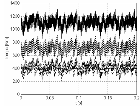
c) Impea, \Psi_{1h} = ct ; f_1 = 5\text{Hz}
