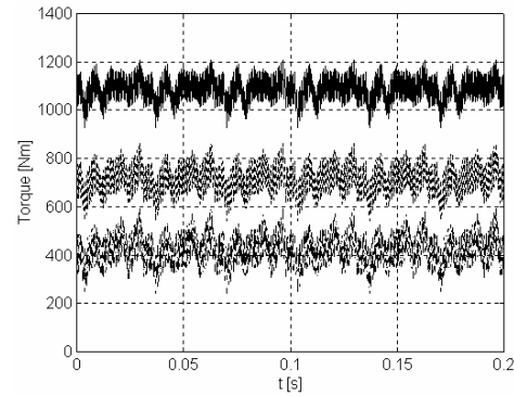
b) Impea, U_1 / f_1 = ct ; f_1 = 5\text{Hz}
